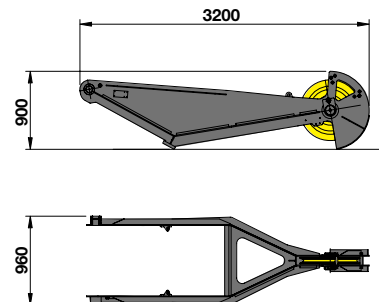
Schnabelausleger: S12.1 auxilliary jib: S12.1
