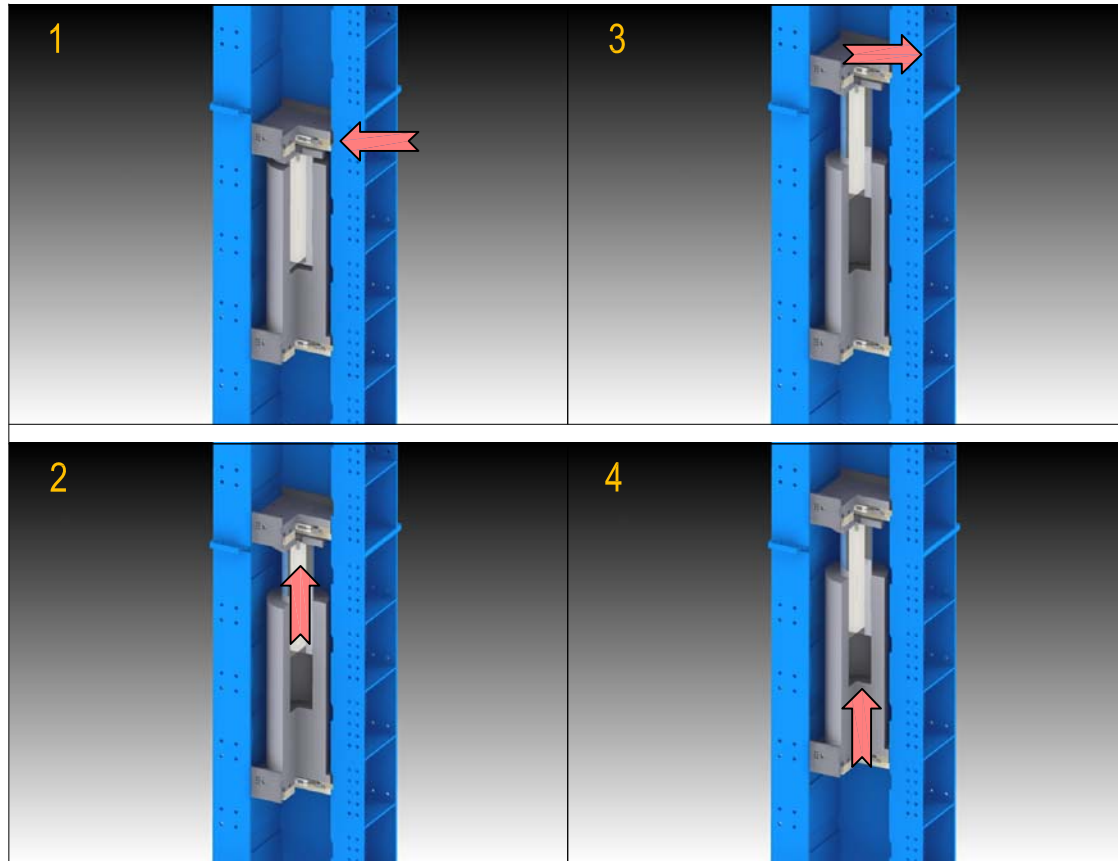
Principle lifting cylindre
