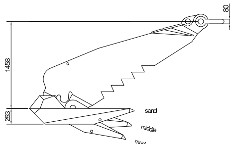
Stevshark
