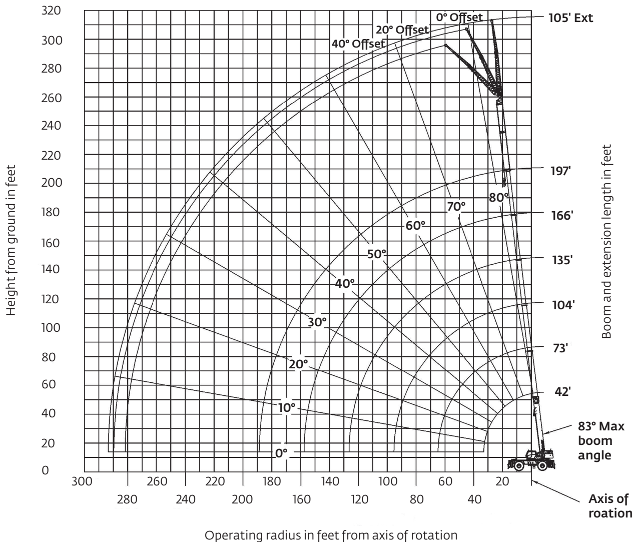
Main boom with bi-fold extension and two inserts
