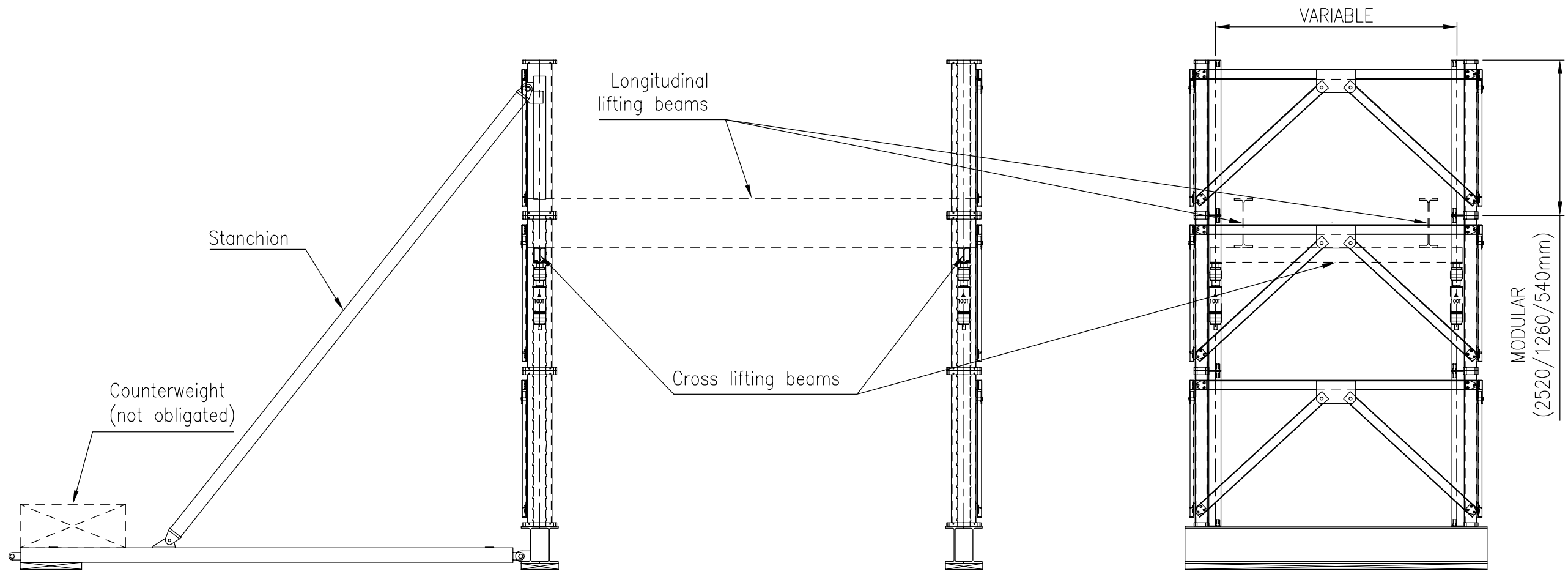
JACKING GANTRY
